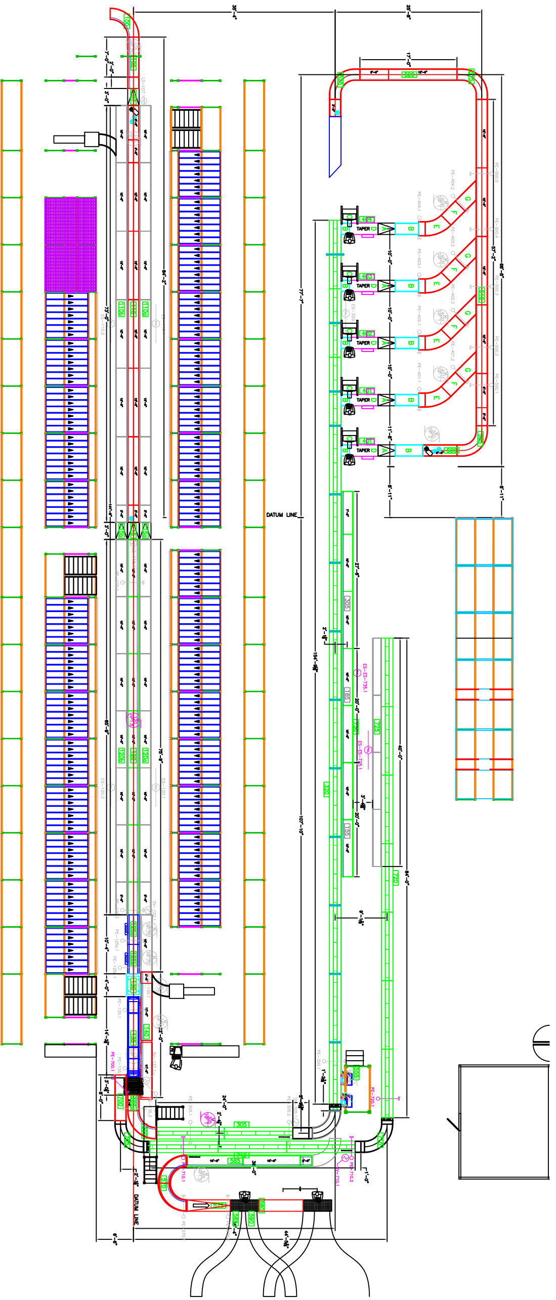
RACK WITH CONVEYOR - FLOOR LEVEL PLAN
